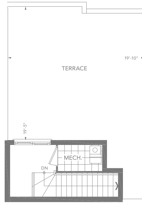
ROOF LEVEL
